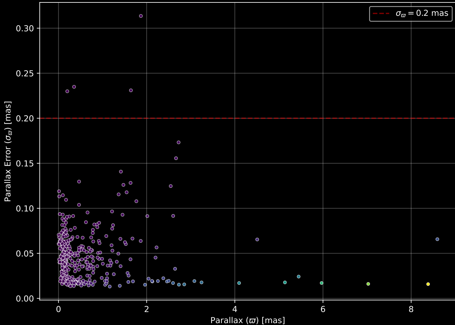
APOGEE DR17 Field: [000+12] Parallax Quality (n= 413)
