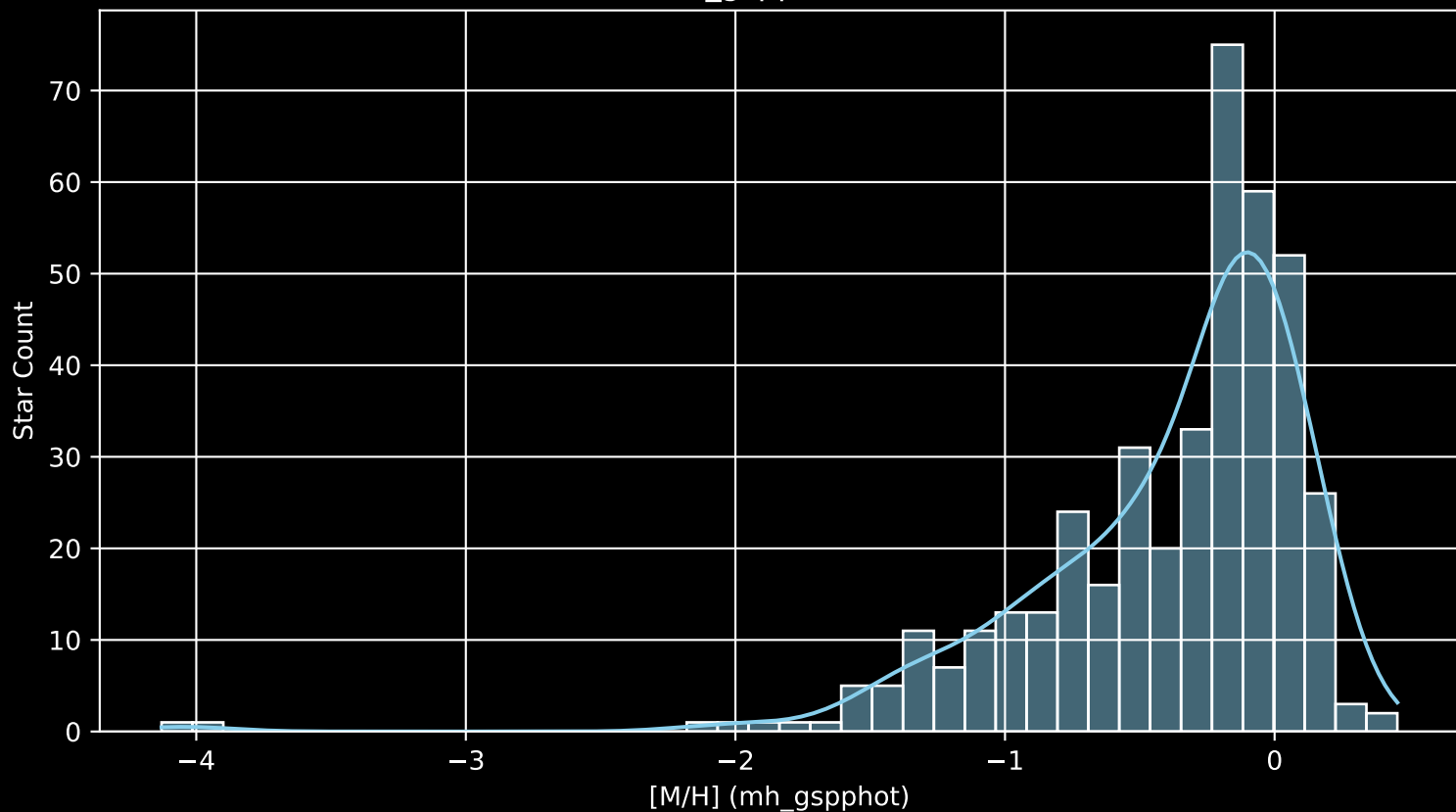
APOGEE DR17 Field: [000+12 [M/H] (mh_gspphot) (n= 413)
