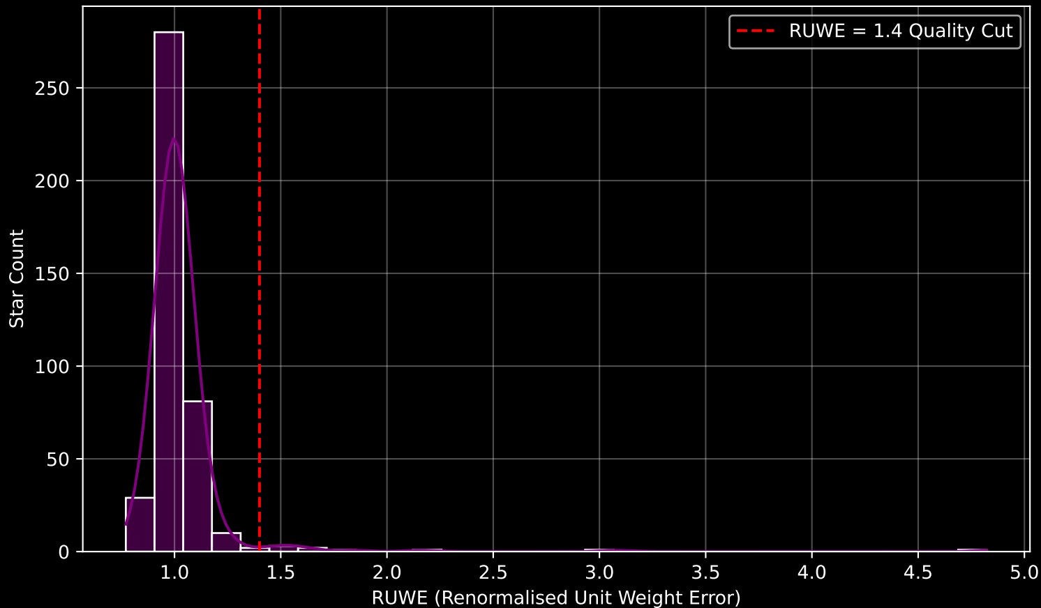
GAPOGEE DR17 Field [000+12] RUWE Distribution (n= 411)
