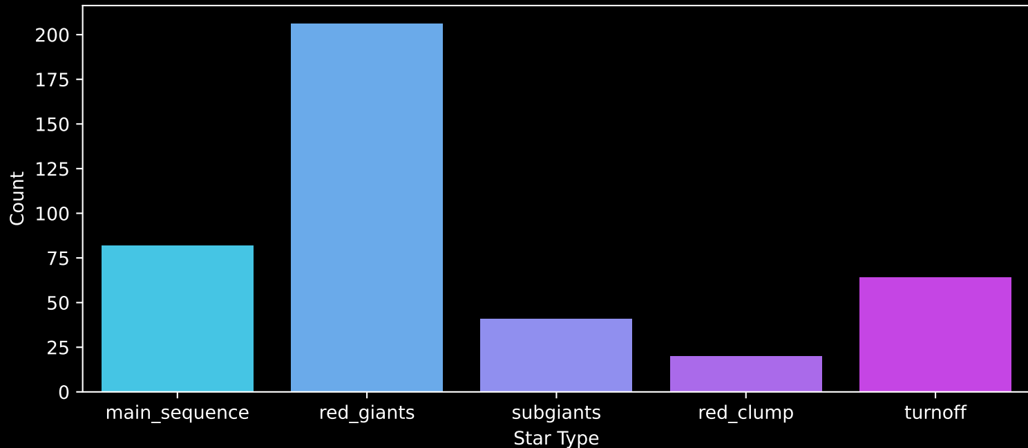
APOGEE DR17 Field: [000+12] Count plot of Star Type
