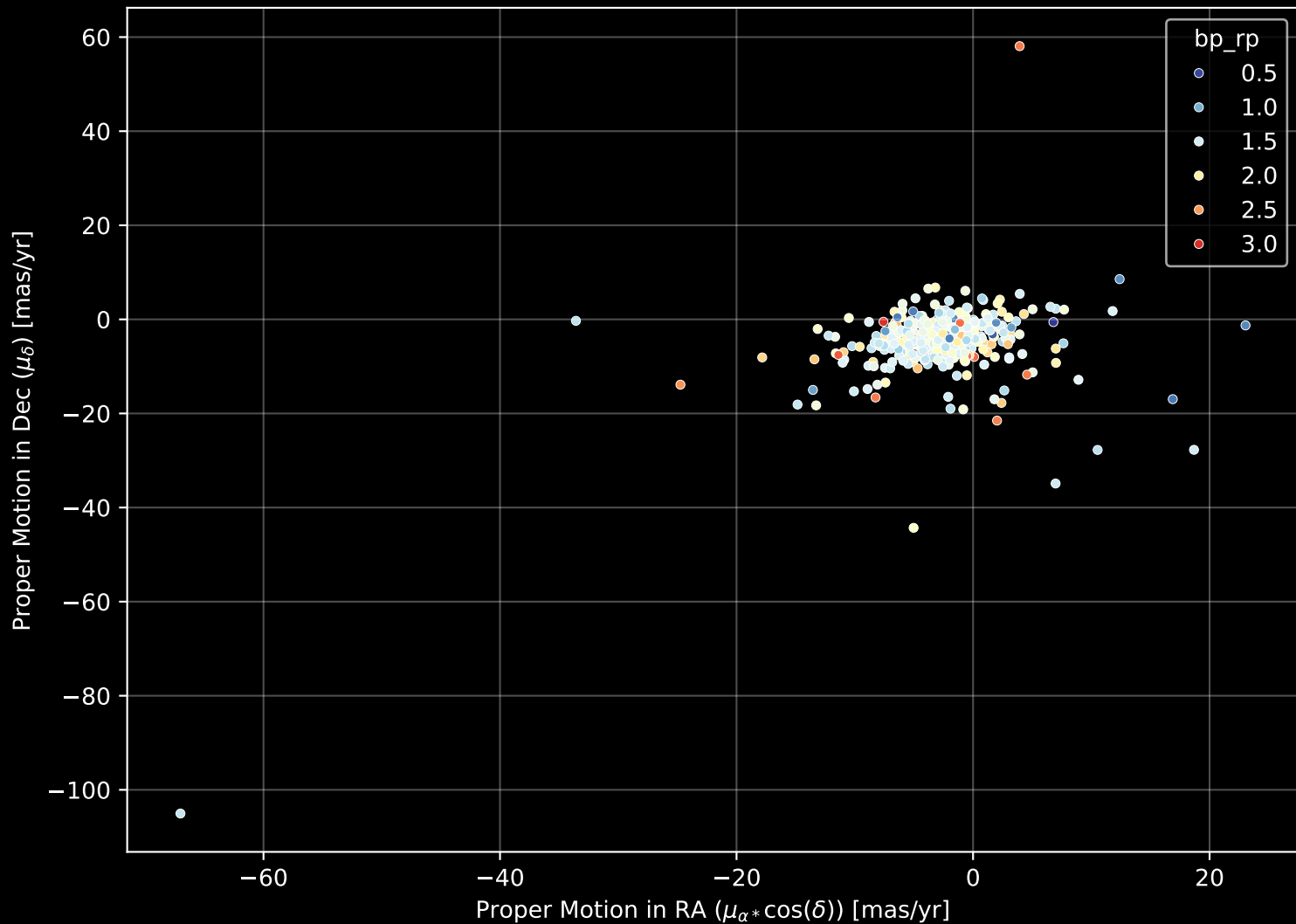
APOGEE DR17 Field: [000+12] Proper Motion Diagram (n= 413)
